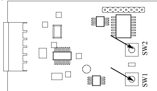
RX-2 Receiver Board
